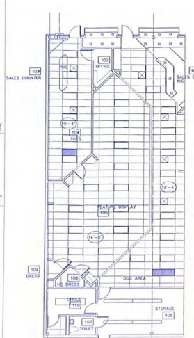
21 REFLECTED CEILING FLOOR PLAN (TYPICAL TENANT)
