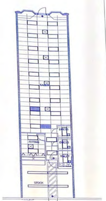
21 REFLECTED CEILING FLOOR PLAN (TYPICAL TENANT)
