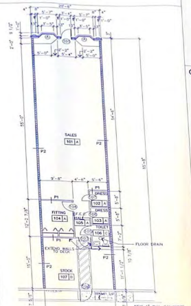
23 FLOOR PLAN
